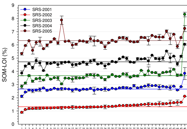
Figure 4. SOM-LOI distribution plots for SRS materials, ALP 2020 Cycle 41.
